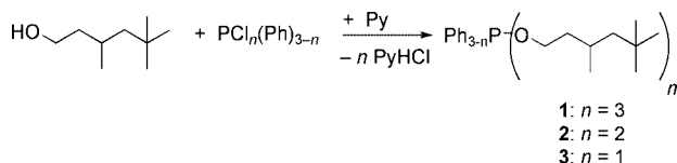
Scheme 1. Synthesis of 1–3.
