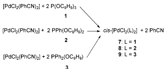
Scheme 3. Syntheses of 7–9 .
