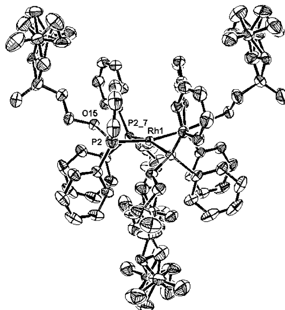
Figure 2. ORTEP drawing of complex 6 . \text{PF}_6^- and hydrogen atoms have been omitted for clarity.
