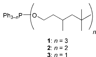
Figure 1. P-donor ligands.
